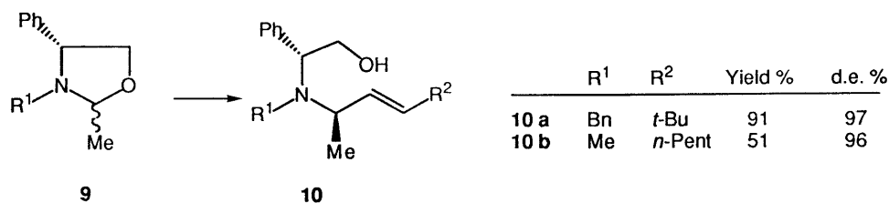
Scheme 3. Reagents and conditions: R 2 –C≡CH, DIBAL, toluene, 4 h, then 9 , 0°C, 1 h
